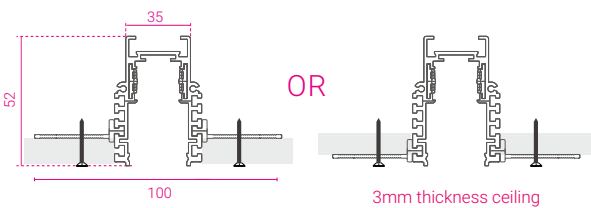
Trimless Recessed Track
