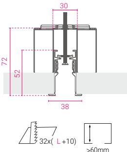
Trim Recessed Track
